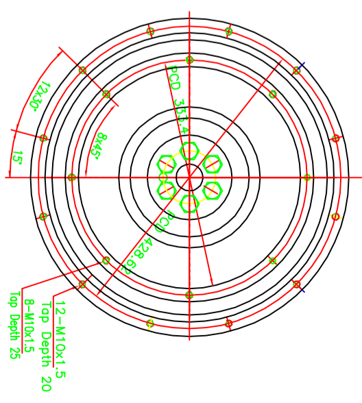
Power Train (S=1.5:1)
